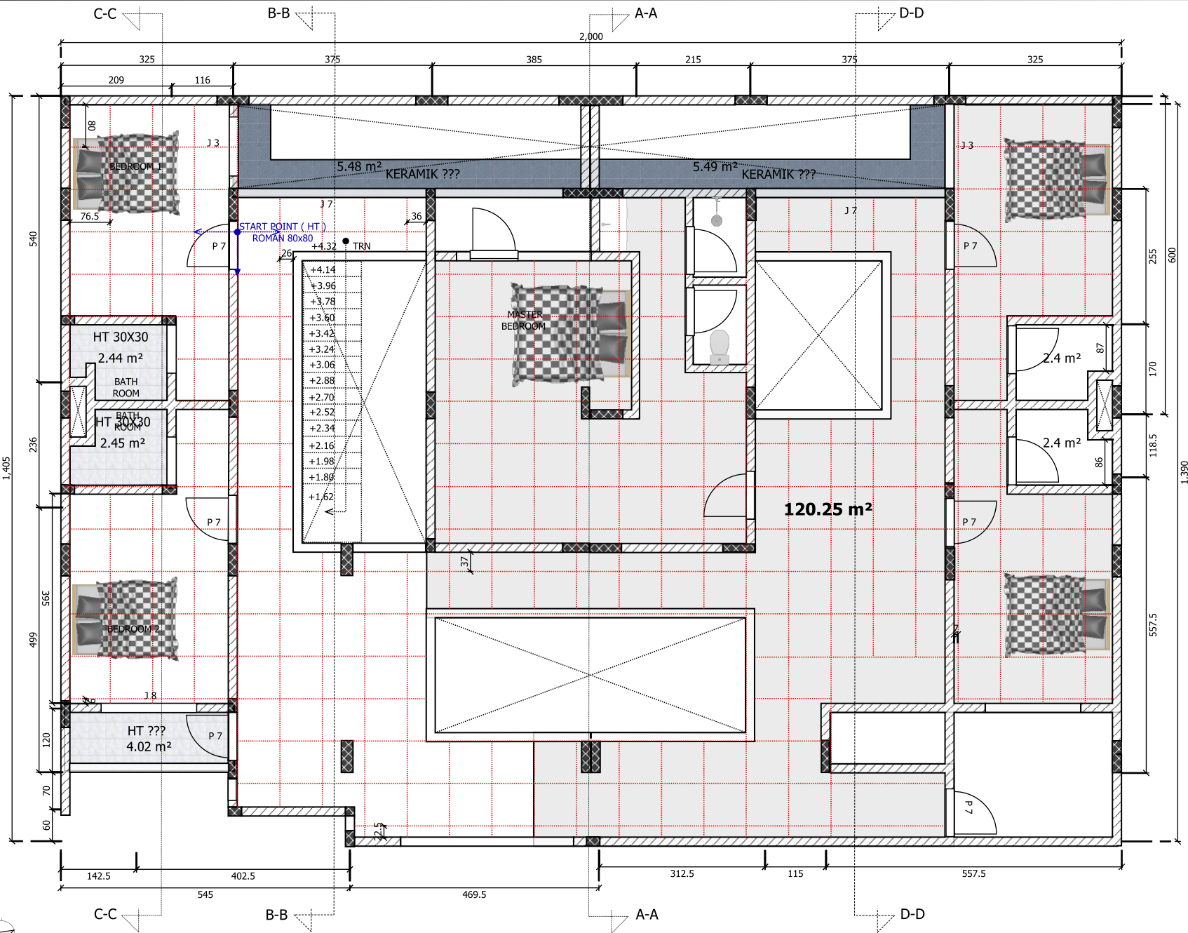
DENAH LANTAI 2 SKALA 1 : 100
