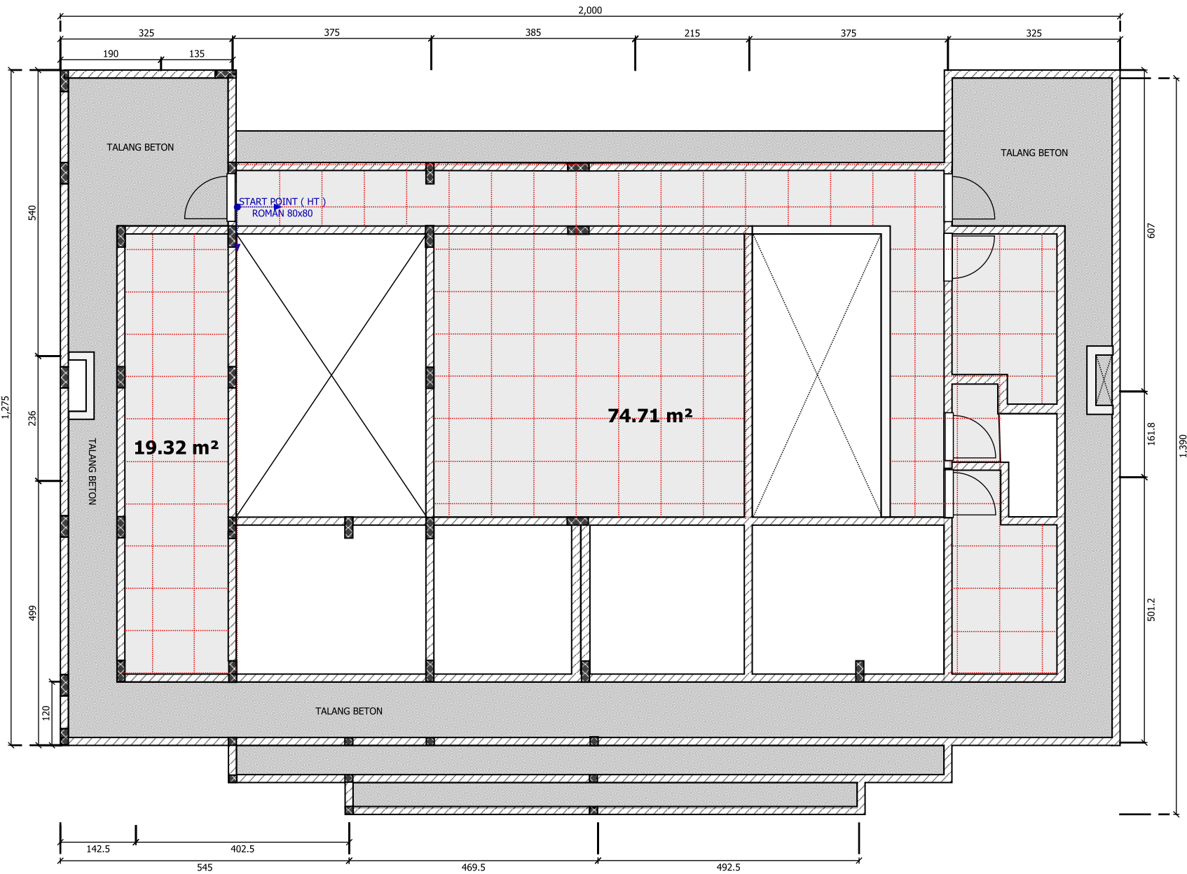
DENAH LANTAI 3 SKALA 1 : 100
