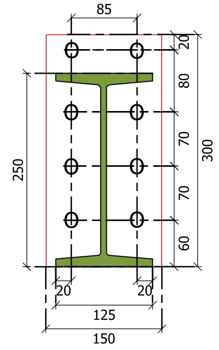
POTONGAN BASE PLATE SKALA 1 : 25
