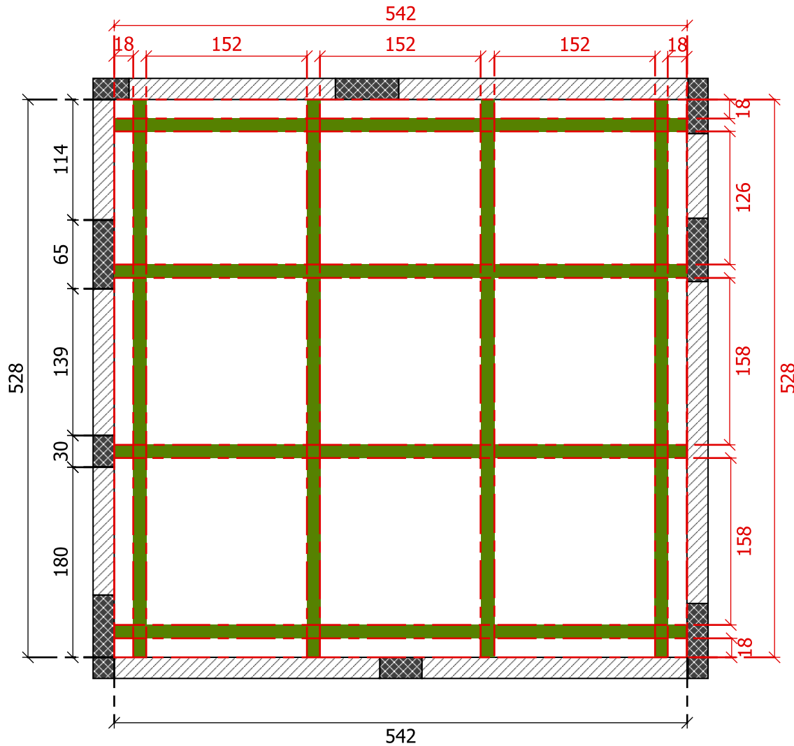
DENAH MEZZANINE SKALA 1 : 50
