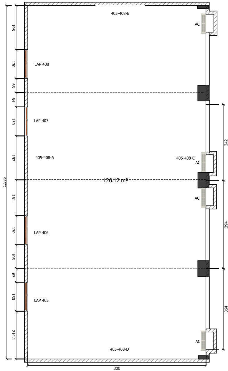
RUANG LAP 405--408 SKALA 1:100
